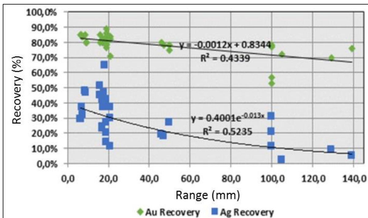
Figure 13-9: Gold and Silver Extraction versus P80 Crush Size
