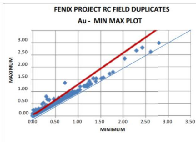
Figure 11-4: Results for all RC Field Duplicates – Au
