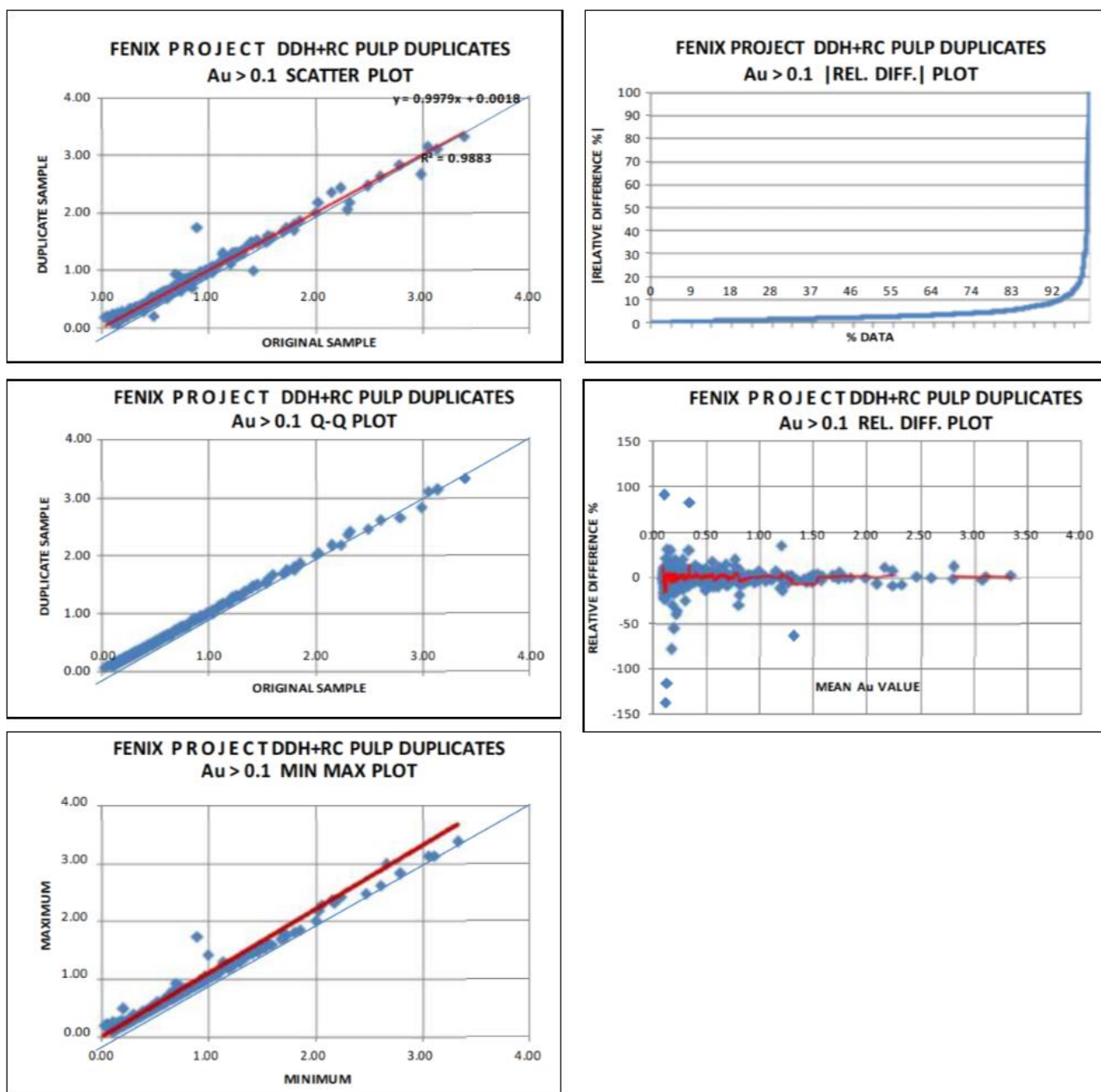
Figure 11-9: Results for the Pulp Duplicates - Au \geq 0.1 ppm
