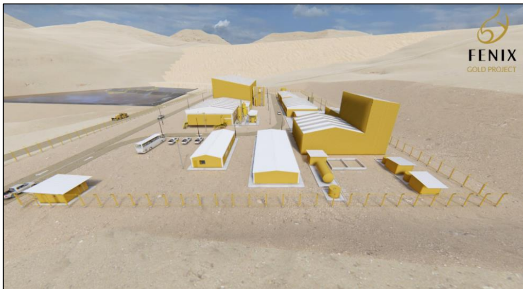
Figure 17-8: Computer generated representation of the ADR plant
