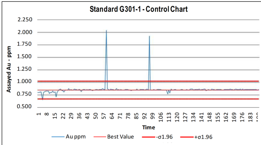
Figure 11-11: Control Chart for Standard G301-1
