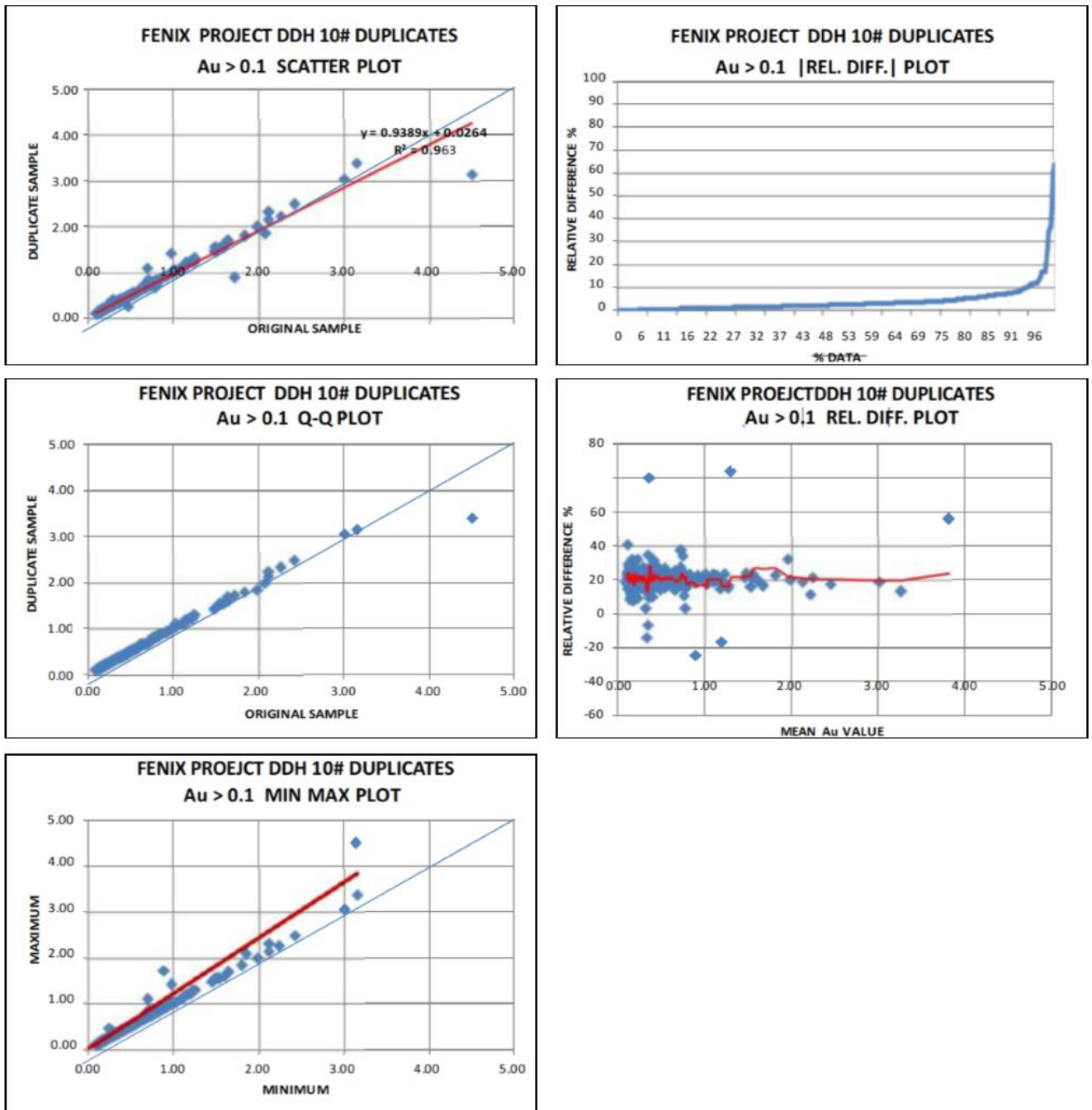
Figure 11-7: Results for the DDH Coarse Duplicates - Au \geq 0.1 ppm
