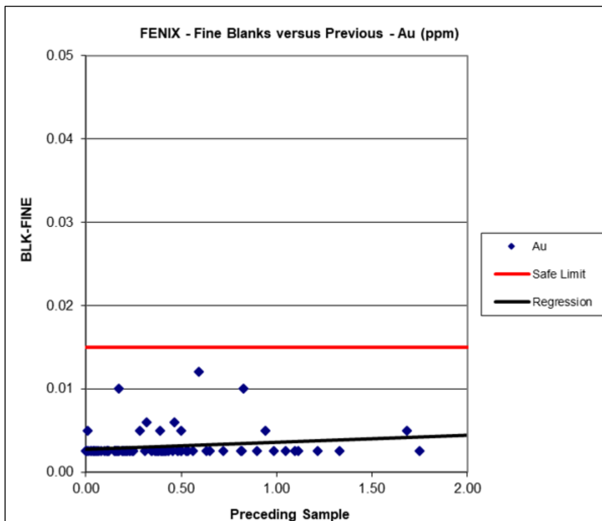
Figure 11-23: Fine Blanks vs Precedent Samples Graph
