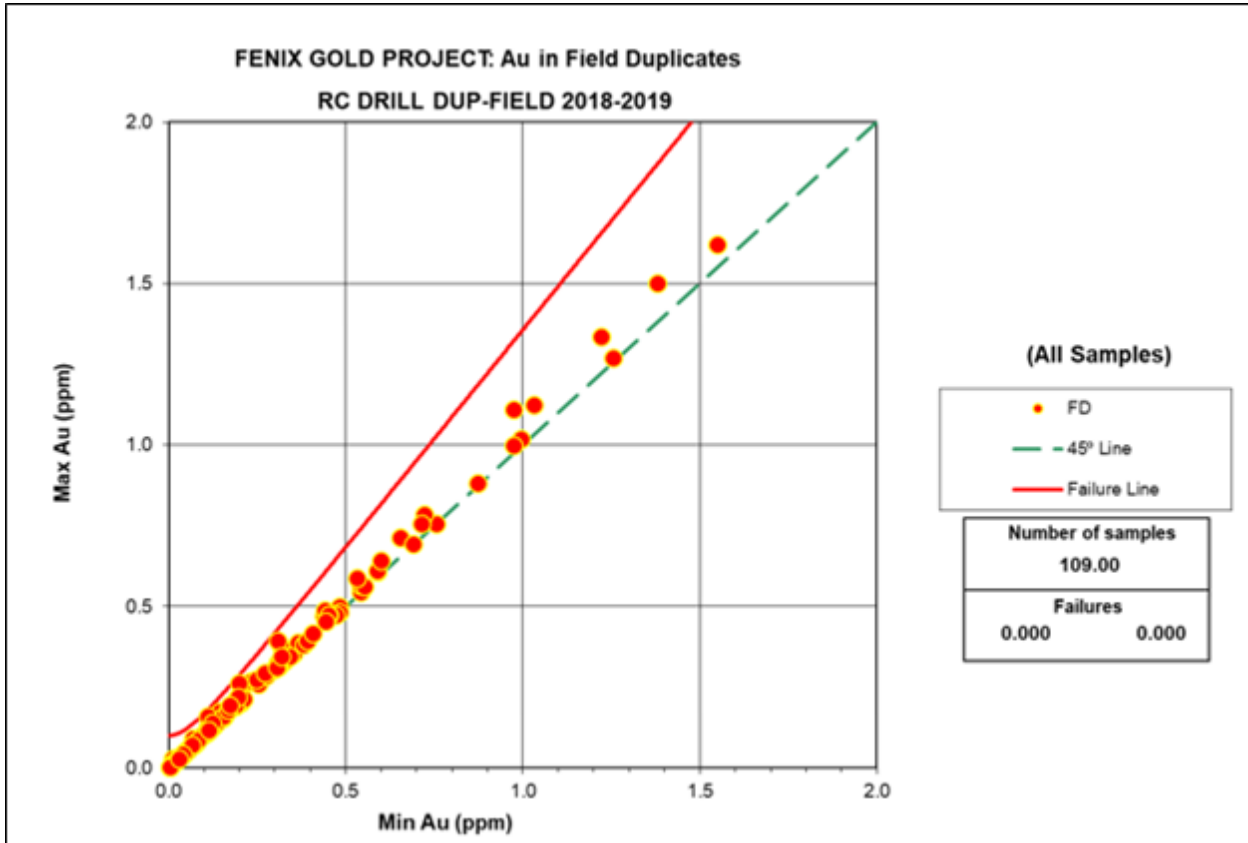
Figure 11-33: Graph Max-Min (Hyperbolic methodology), for field duplicates (DUP-FIELD) RC drill holes
