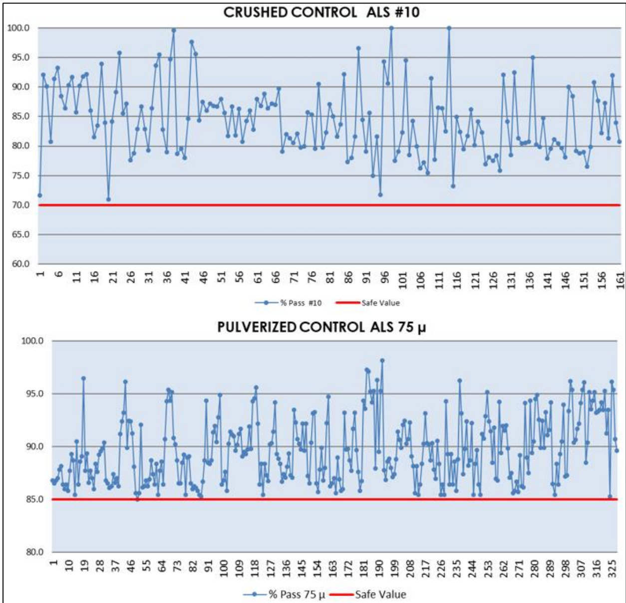
Figure 11-22: Granulometric control graphs for crushing and pulverized stages
