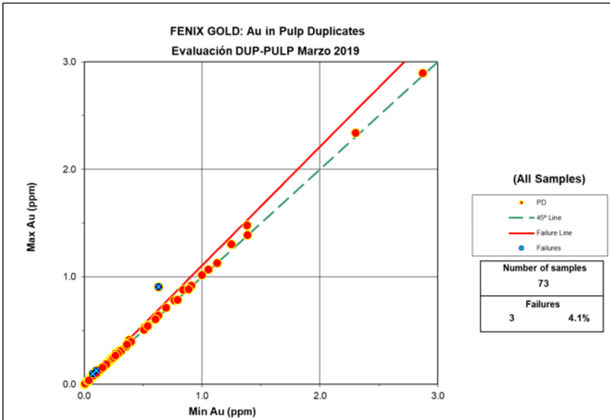
Figure 11-36: Graph Max-Min for pulp Duplicates
