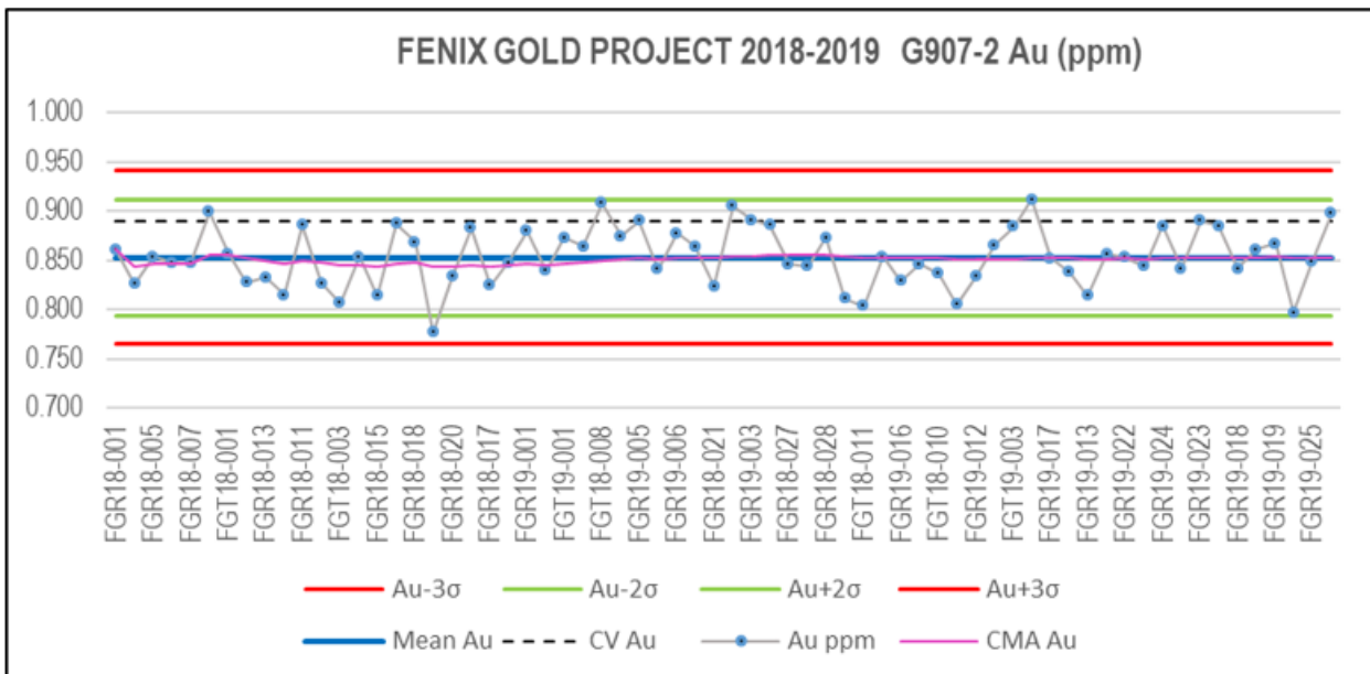
Figure 11-29: Graphic for Standard G907-2
