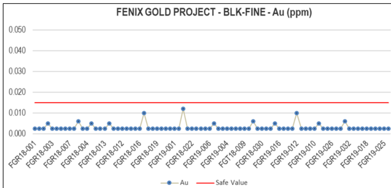
Figure 11-24: Fine Blank Graphs in time periods
