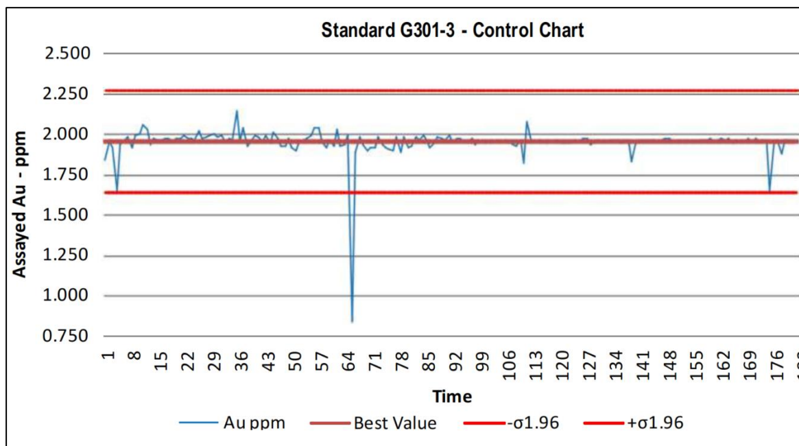
Figure 11-12: Control Chart for Standard G301-3
