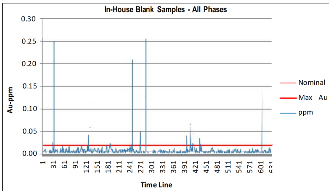
Figure 11-17: Time Sequenced Au Values – In House Blanks
