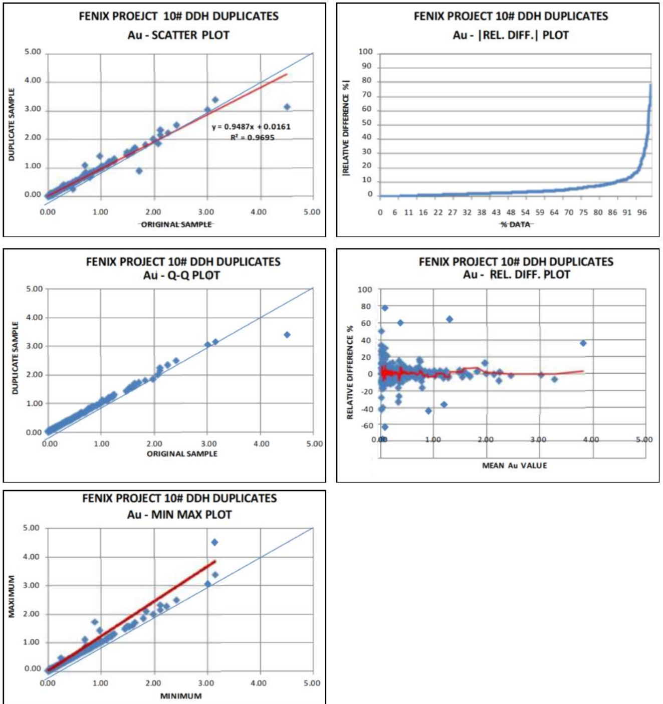
Figure 11-6: Results for DDH Coarse Duplicates – Au
