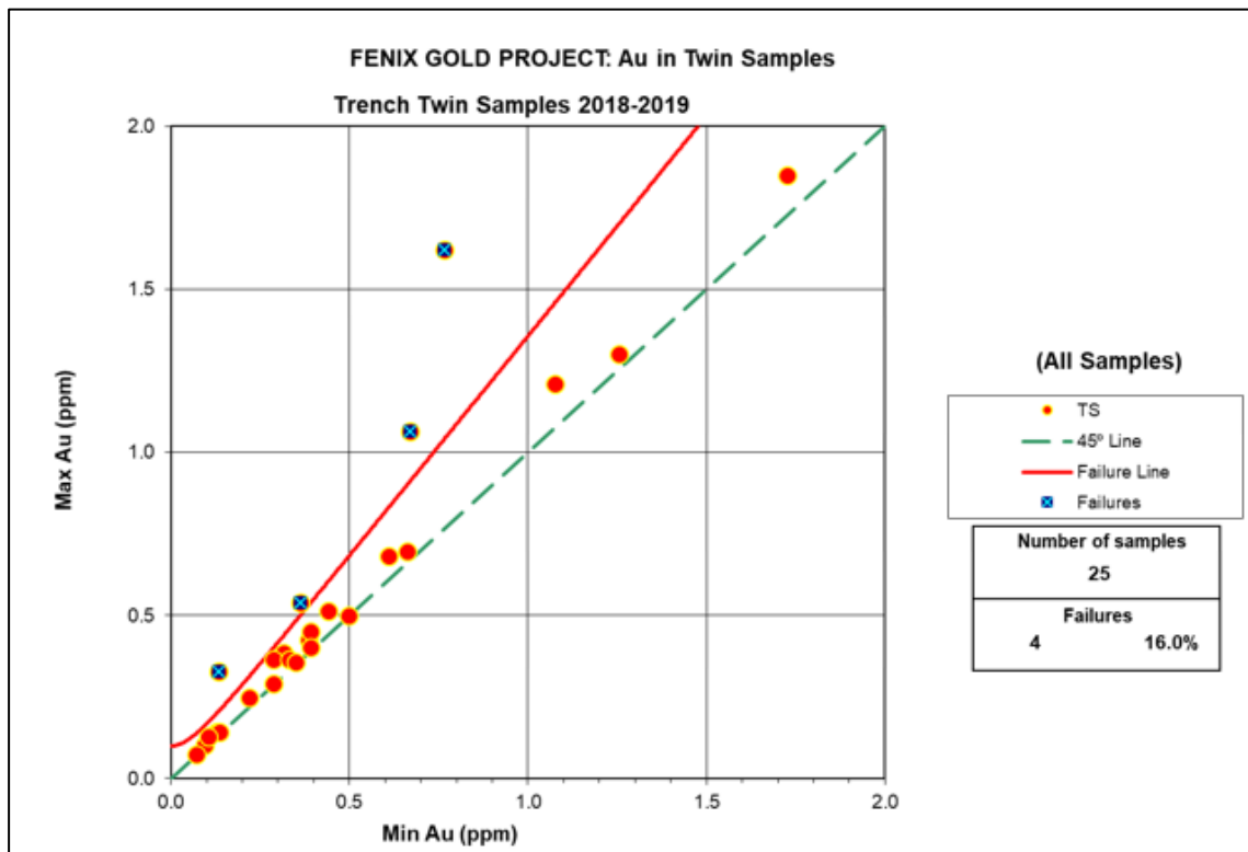
Figure 11-34: Graph Max-Min (Hyperbolic methodology), for twin Duplicates (Twin Samples), trench
