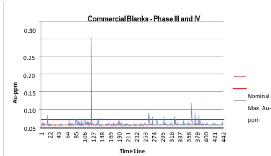
Figure 11-19: Geostats Pty Ltd Blank Certified Material - Gold Values
