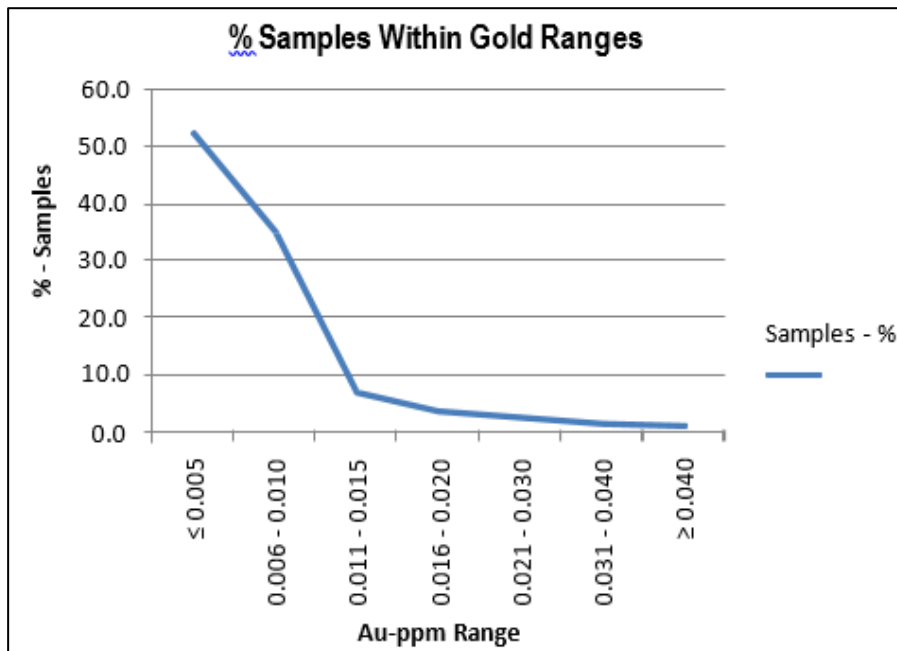
Figure 11-20: Geostats Pty Ltd Blank Certified Material - Frequency Plot
