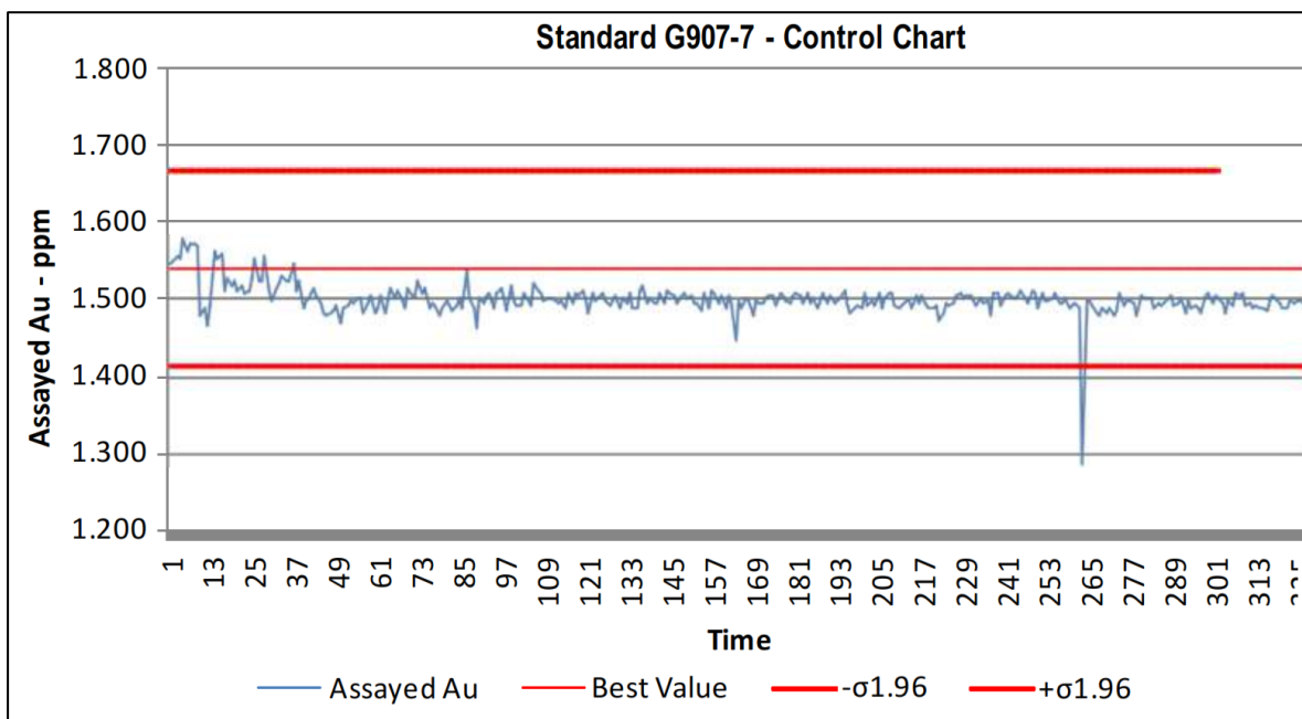
Figure 11-16: Control Chart for Standard G907-7
