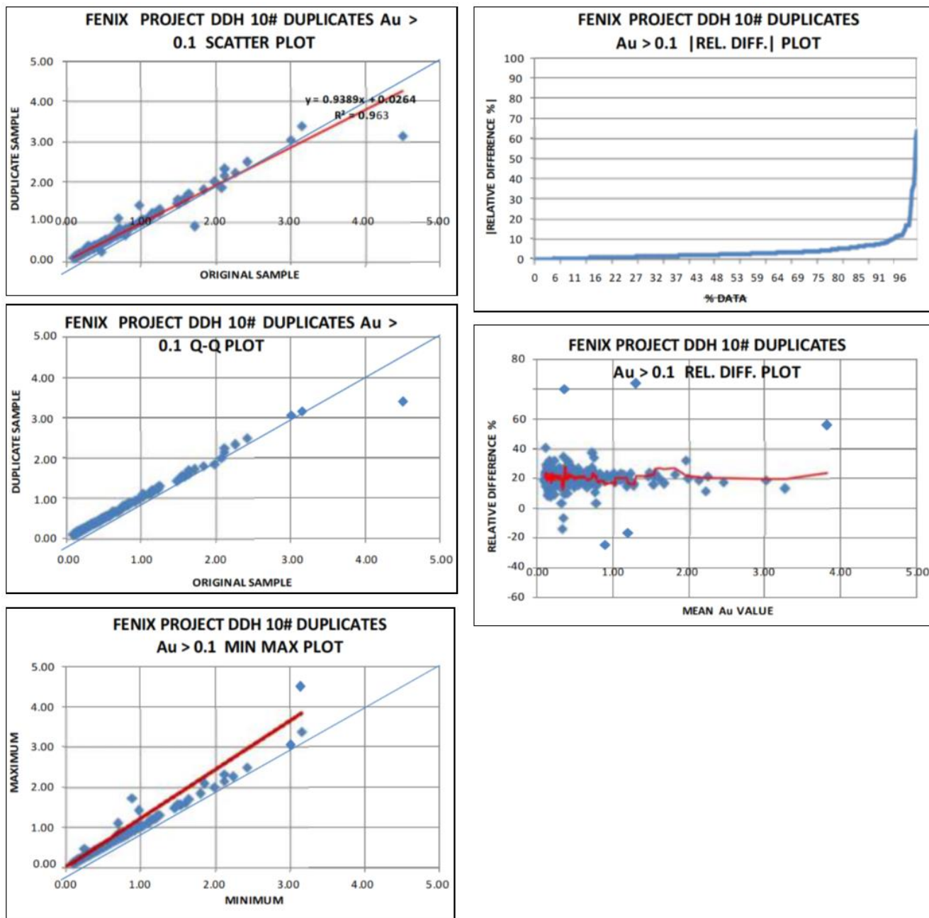
Figure 11-8: Results for all Pulp Duplicates – Au
