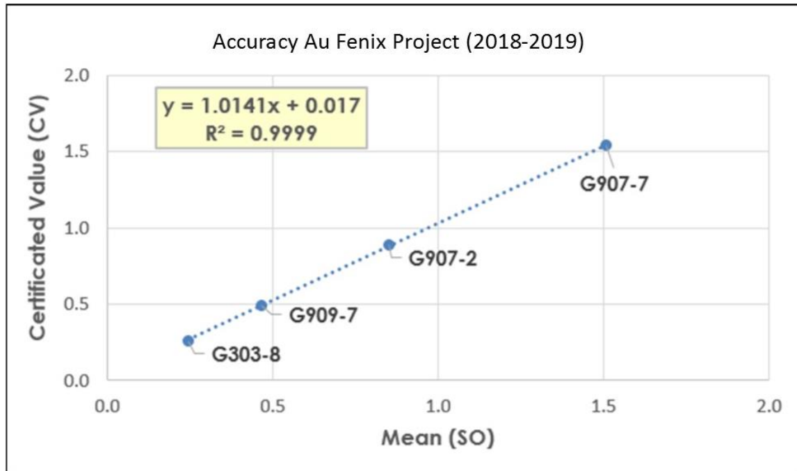
Figure 11-31: Linear Regression for Global Bias Calculation
