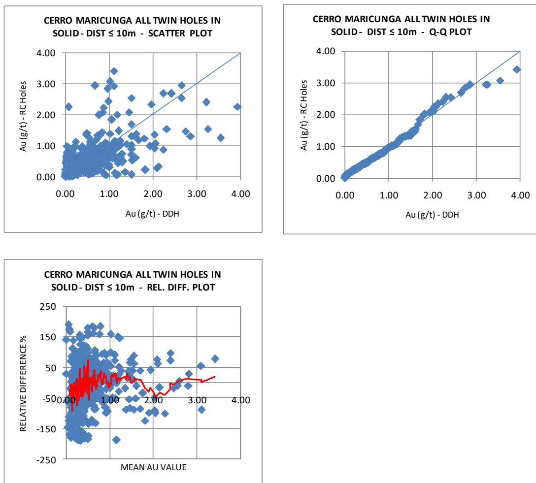
Figure 11-21: Statistical Plots for DDH & RC Twin Holes
