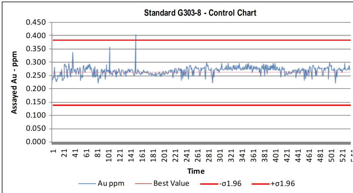
Figure 11-13: Control Chart for Standard G303-8
