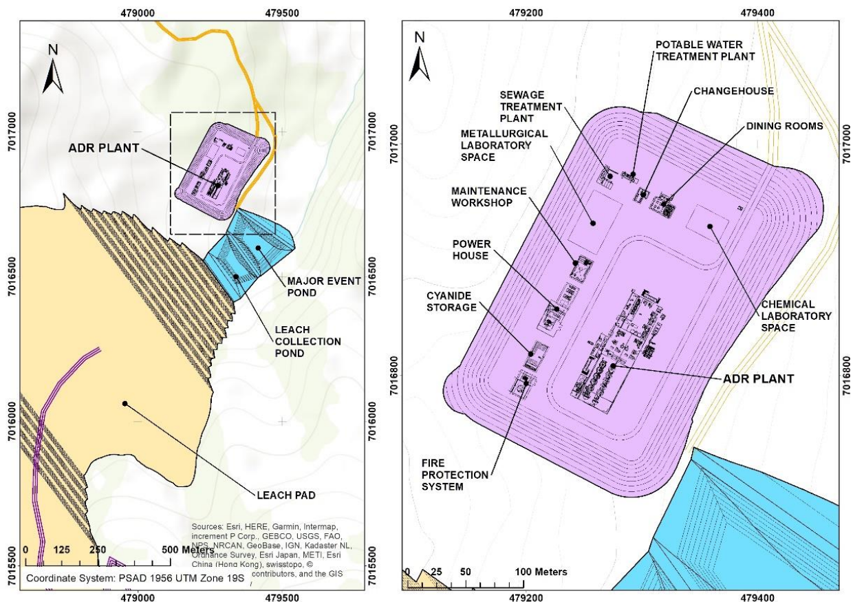
Figure 18-6: Plant Infrastructure
