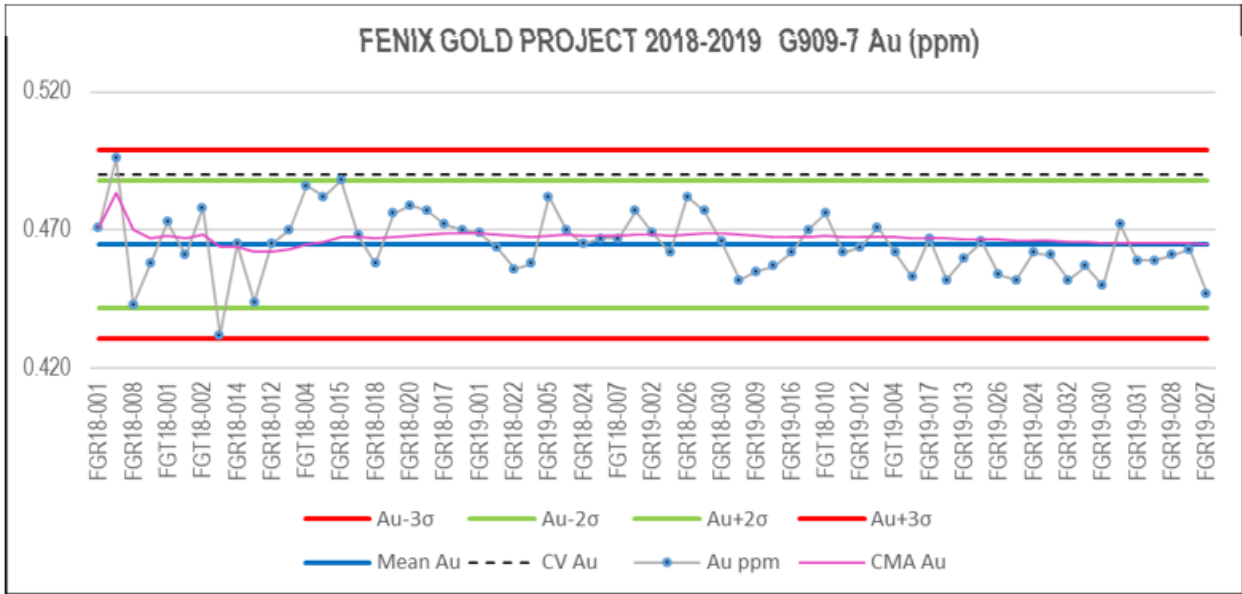
Figure 11-28: Graphic for Standard G909-7
