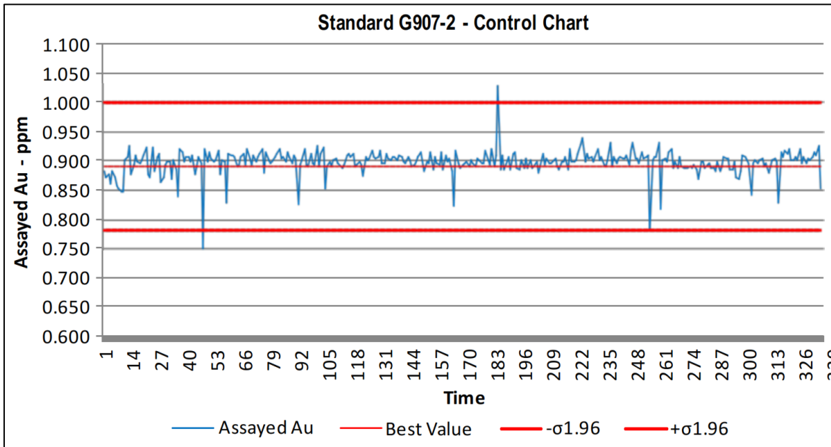
Figure 11-15: Control Chart for Standard G907-2
