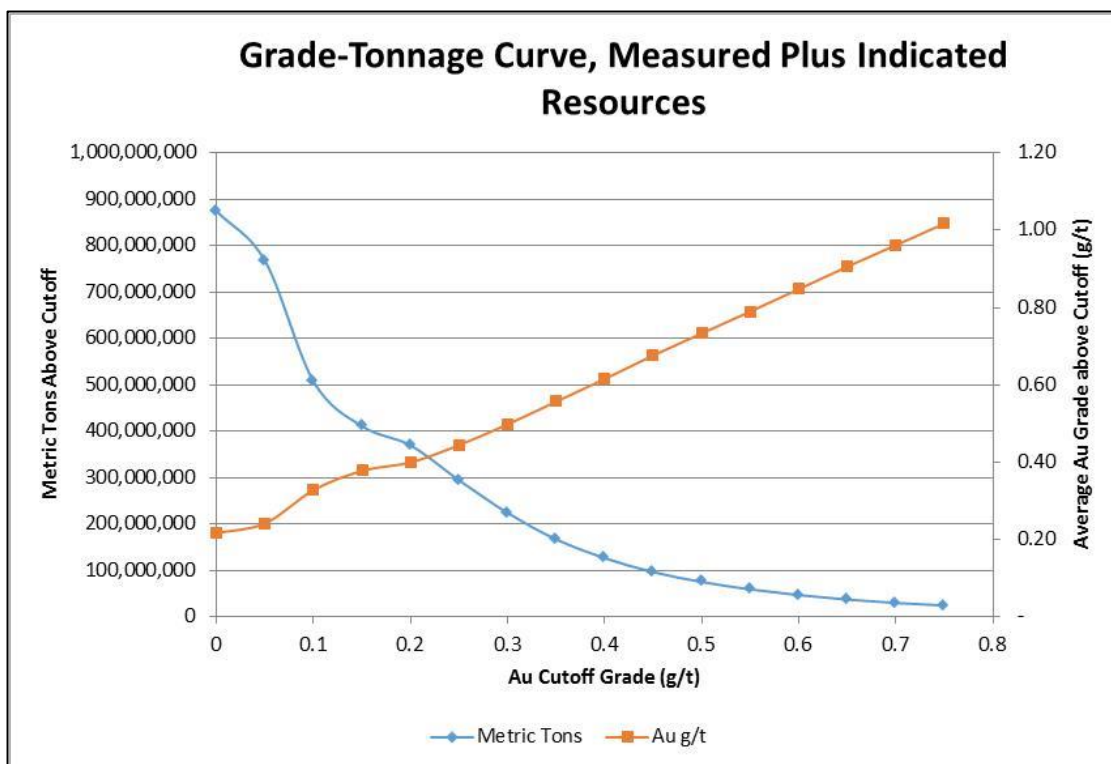
Figure 14-32: Grade-Tonnage Curve, Measured + Indicated Resources, Fenix Gold Project
