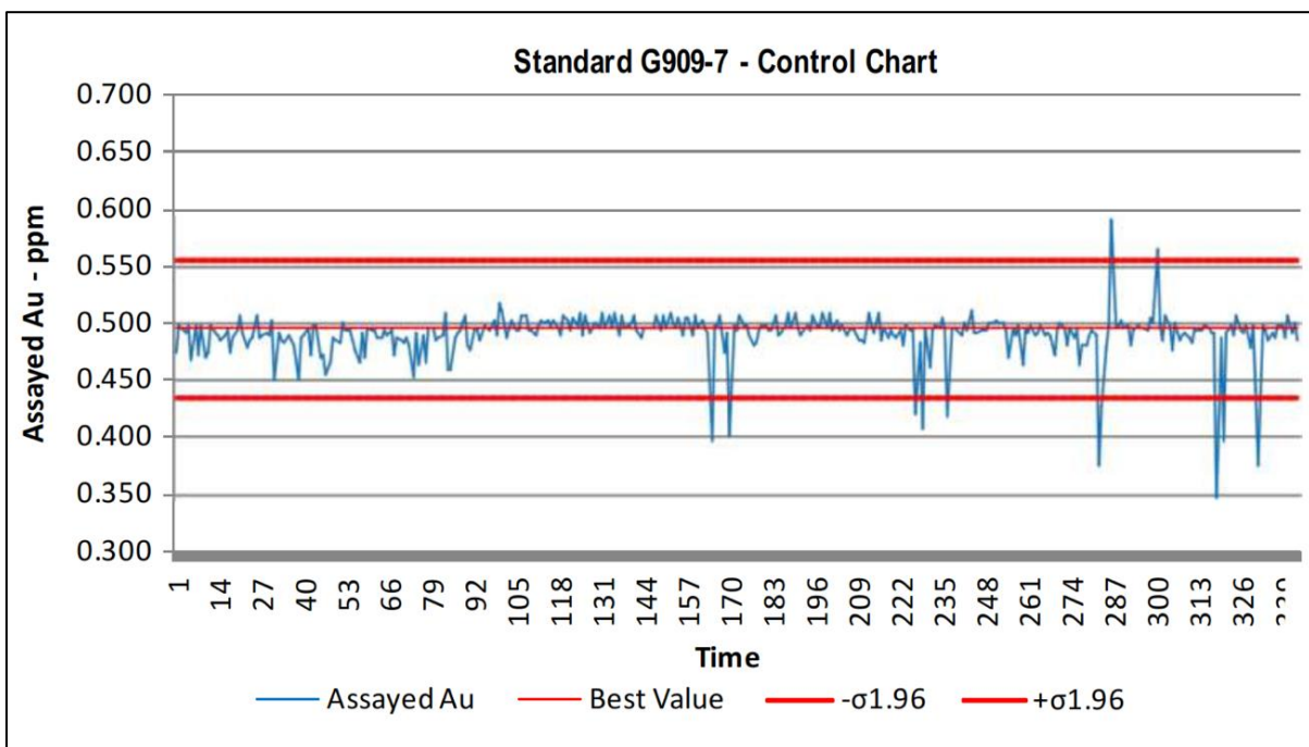
Figure 11-14: Control Chart for Standard G909-7
