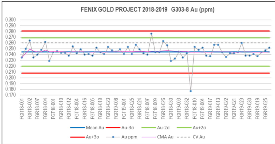
Figure 11-27: Graphic for Standard G303-8
